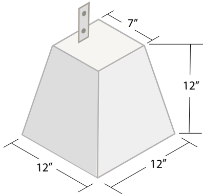
12" Garage Pier with Strap ITEM #127GPS
