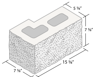
6 x 8 x 16 Split L-Return
