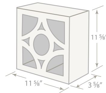
#1086 Screen Block 4 x 12 x 12
