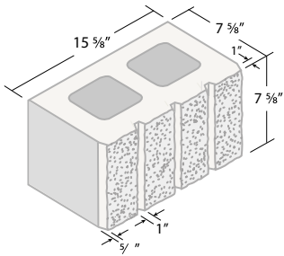
8 x 8 x 16 3V Fluted Split, 1 Face* ITEM #0883V
