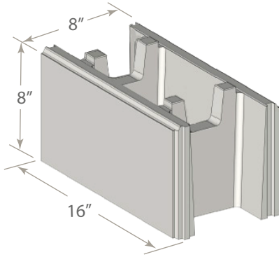
Tileco Mortarless Block Runner 8 x 8 x 16 ITEM #H088R
