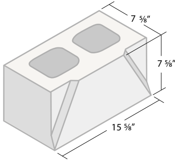
8 x 8 x 16 Shadowcaster Center*
