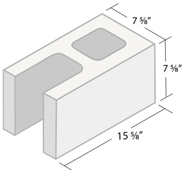
8 x 8 x 16 Plumber ITEM #088P
