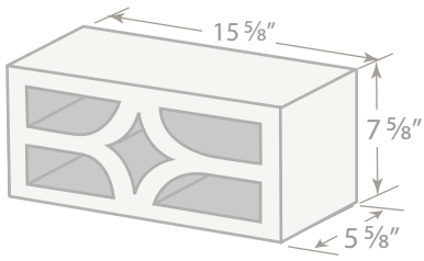
#422 6" Screen Block 6 x 8 x 16 ITEM #6S422
