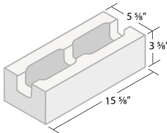
6 x 4 x 16 Bond Beam* ITEM #064K
