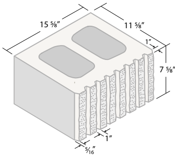
12 x 8 x 16 7V Fluted Split 1 Face** ITEM #0887V
