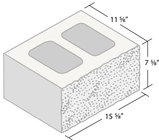
12 x 8 x 16 Split 1 Face ITEM #128S
