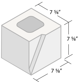
8 x 8 x 8 Shadowcaster Left Half*
