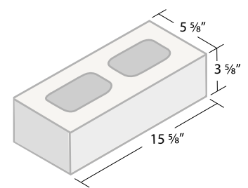
6 x 4 x 16 Double Solid End ITEM #064D
