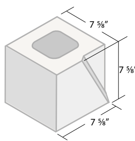
8 x 8 x 8 Shadowcaster Right Half*
