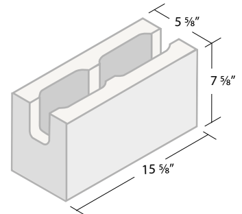
6 x 8 x 16 Bond Beam ITEM #068K
