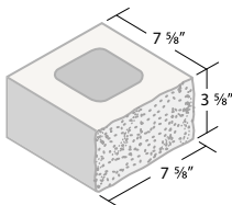
8 x 4 x 8 Split Half, 1 Face* ITEM #084SH
