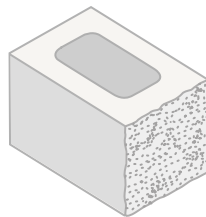
12 x 8 x 8 Split Half, 1 Face* ITEM #128SH
