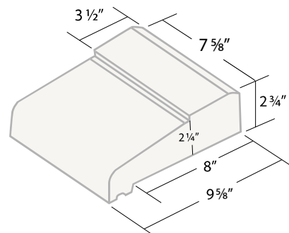
8" Window Sill J-2
