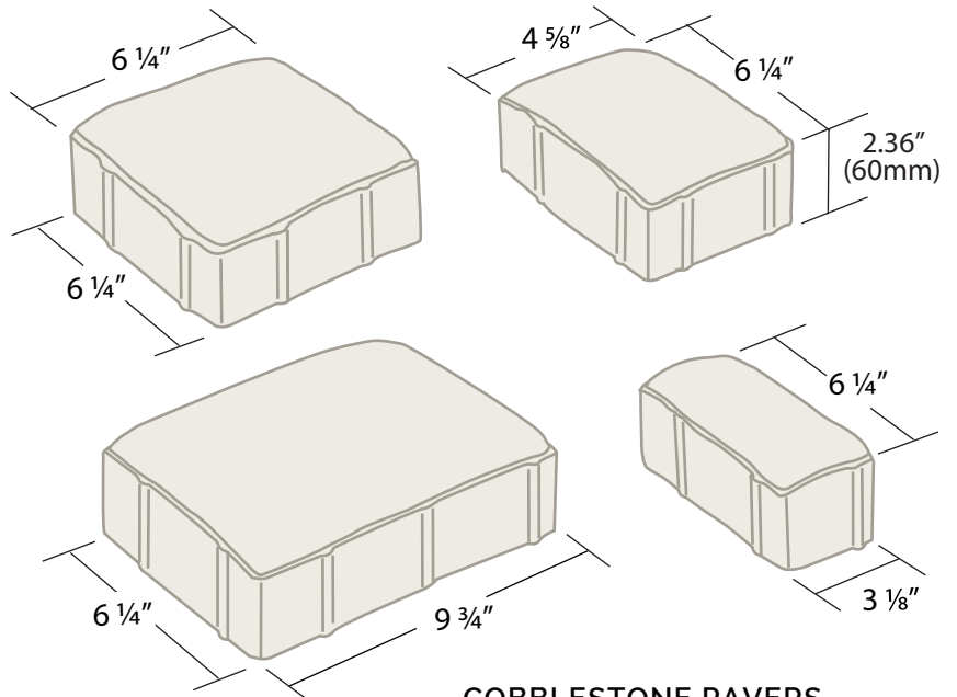
COBBLESTONE PAVERS (available in Black, Gray, Red and Tan)
