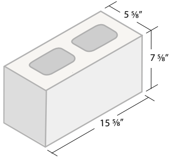
6 x 8 x 16 Double Solid End ITEM #068D
