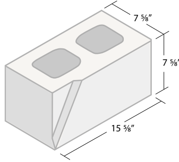
8 x 8 x 16 Shadowcaster Left*
