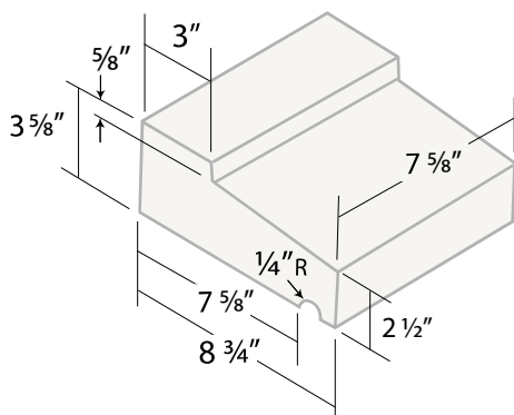
9" Window Sill J-3
