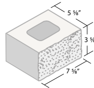
6 x 4 x 8 Split Half, 1 Face*
