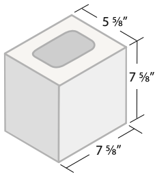
6 x 8 x 8 Half ITEM #068H
