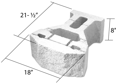
STANDARD I Tri-plane Split Face (available in Basalt or Limestone)
