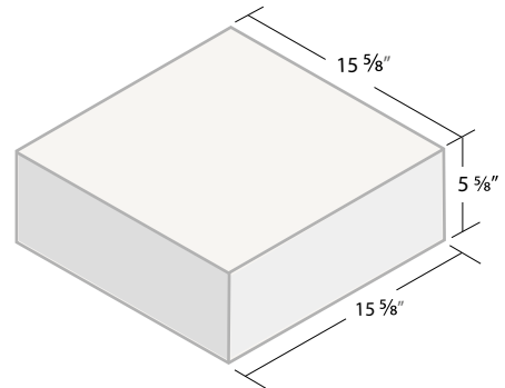
16 x 6 x 16 Foundation Block ITEM #166F
