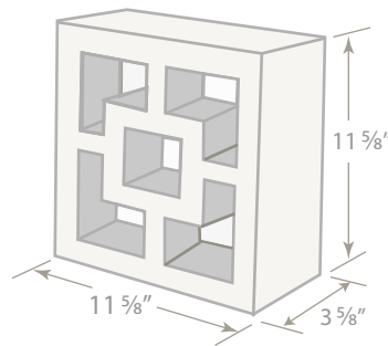
#397 Screen Block 4 x 12 x 12
