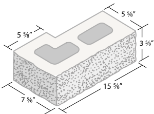
6 x 4 x 16 Split L-Return*
