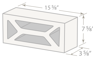
#314 4" Screen Block 4 x 8 x 16 ITEM #4S314
