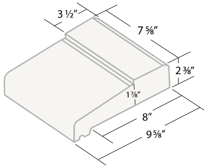
8" Window Sill J-1
