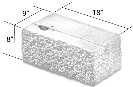
KEYKUT RIGHT CORNER Straight Keycut Face (available in Dark Gray, Tan, Rose, or Limestone Keykut)
