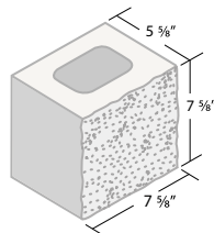
6 x 8 x 8 Split Half, 1 Face*
