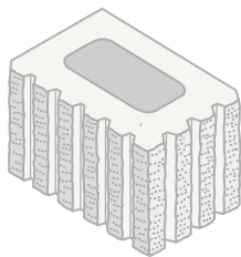
12 x 8 x 8 7V Fluted Split 1 Face / 1 End Half** ITEM #0887VK
