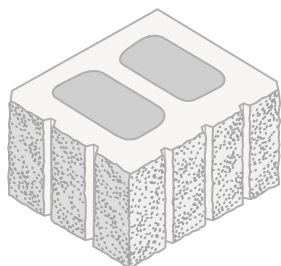
12 x 8 x 16 3V Fluted Split 1 Face / 1 End** ITEM #1283VFE
