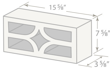
#422 4" Screen Block 4 x 8 x 16 ITEM #4S422
