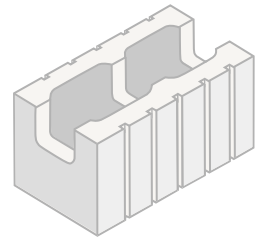
8 x 8 x 16 5-Score Bond Beam, 2 Face** ITEM #0885GFFK
