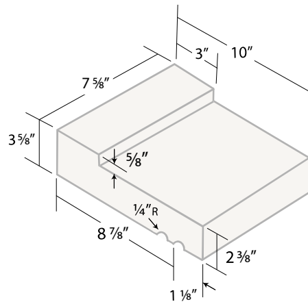
10" Window Sill J-4
