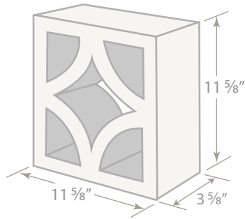
#377 Screen Block 4 x 12 x 12
