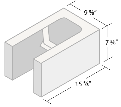
10 x 8 x 16 Single Open End* ITEM #108SOE
