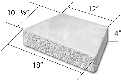
UNIVERSAL CAP Straight Keycut Face (available in Dark Gray, Tan, Rose, or Limestone Keykut)
