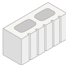
6 x 8 x 16 5-Score DSE** ITEM #0685GD
