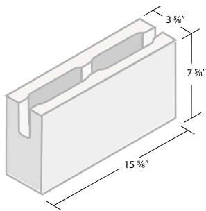
4 x 8 x 16 Bond Beam ITEM #048K
