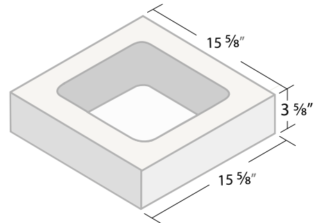
16 x 4 x 16 Column* ITEM #164C
