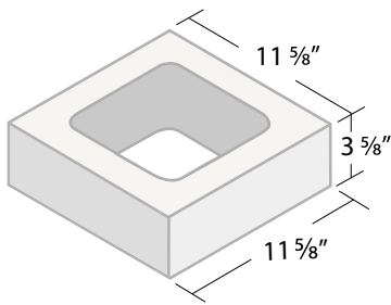
12 x 4 x 12 Column* ITEM #124C
