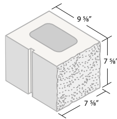
10 x 8 x 8 Split Jamb Half, 1 Face** ITEM #108SJH
