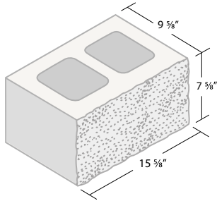
10 x 8 x 16 Split 1 Face** ITEM #108S
