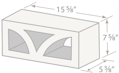
#414 6" Screen Block 6 x 8 x 16 ITEM #6S414
