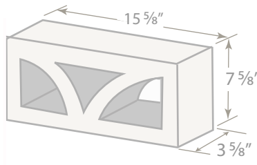
#414 4" Screen Block 4 x 8 x 16 ITEM #4S414
