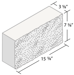
4 x 8 x 16 Split (Solid) 1 Face Veneer**
