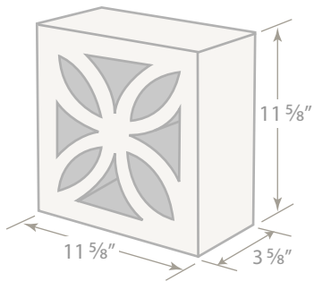
#399 Screen Block 4 x 12 x 12
