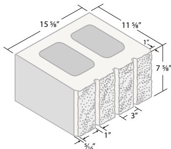
12 x 8 x 16 3V Fluted Split 1 Face** ITEM #1283V
