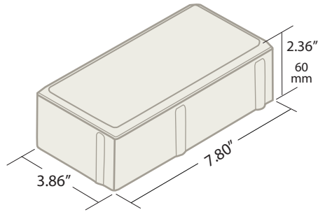
CLASSIC PAVER 60mm (available in Gray, Red and Tan)
