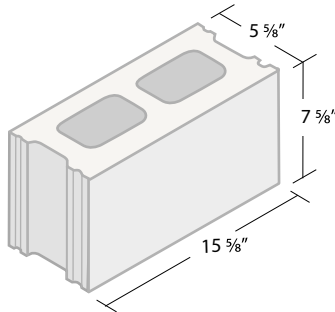
6 x 8 x 16 Runner ITEM #068M
