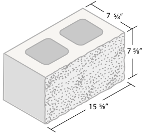
8 x 8 x 16 Split 1 Face ITEM #088S
