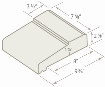
8" WINDOW SILL J-1
