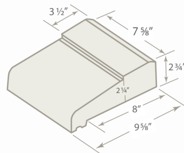
8" WINDOW SILL J-2
