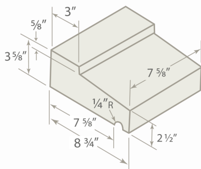
WINDOW SILL J-3
