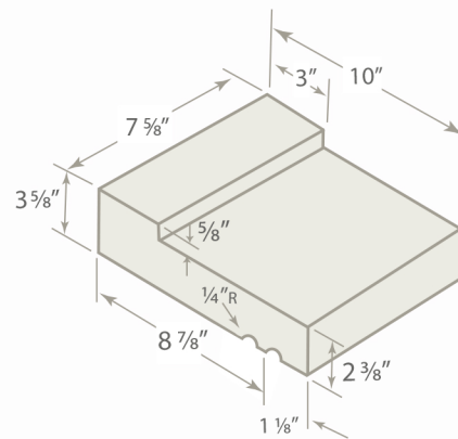
WINDOW SILL J-4
