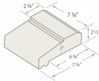
6" WINDOW SILL
