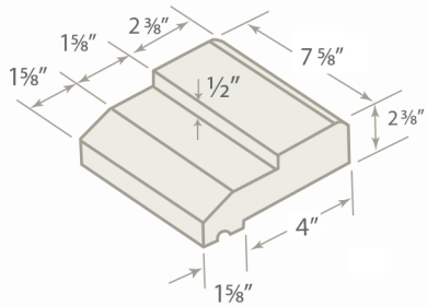
4" WINDOW SILL
