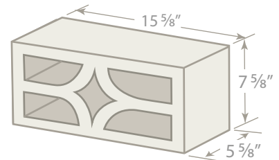
#422 6" SCREEN BLOCK 6x8x16
