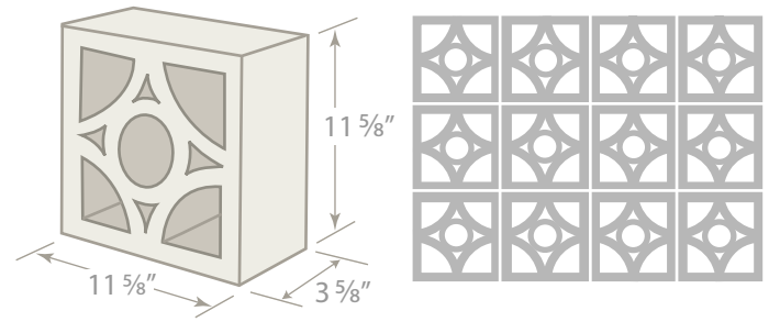
#1086 SCREEN BLOCK 4x12x12
