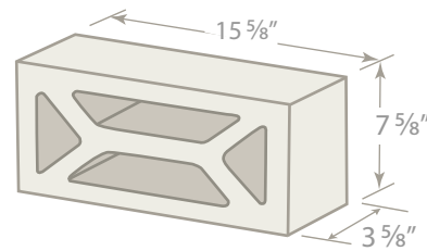
#314 4" SCREEN BLOCK 4x8x16
