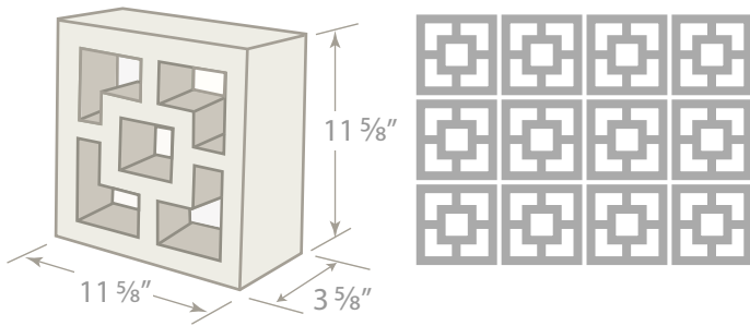
#397 SCREEN BLOCK 4x12x12
