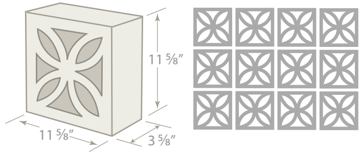
#399 SCREEN BLOCK 4x12x12
