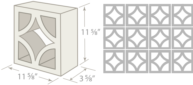
#377 SCREEN BLOCK 4x12x12
