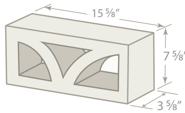
#414 4" SCREEN BLOCK 4x8x16
