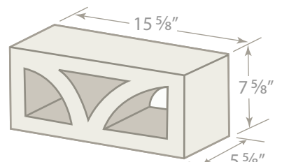
#414 6" SCREEN BLOCK 6x8x16
