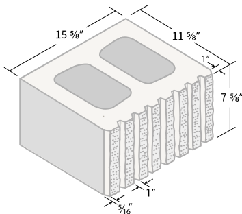
12 x 8 x 16 7V Fluted Split 1 Face** ITEM #1287V
