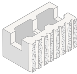
8 x 8 x 16 7V Fluted Split Bond Beam, 1 Face* ITEM #0887VK
