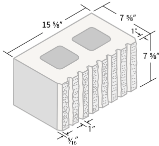
8 x 8 x 16 7V Fluted Split, 1 Face* ITEM #0887V
