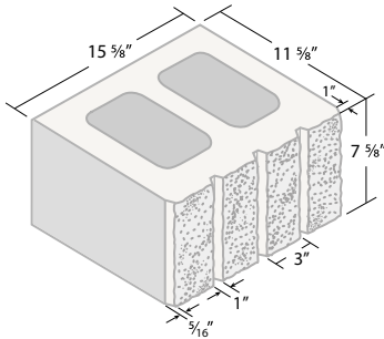
12 x 8 x 16 3V Fluted Split 1 Face**
